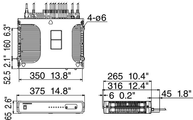
FELCOM250/500 Communication Unit FB-2000 4.1 kg 9 lb
