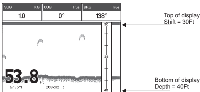
Figure 17.8.2 - Example of Depth and Shift
