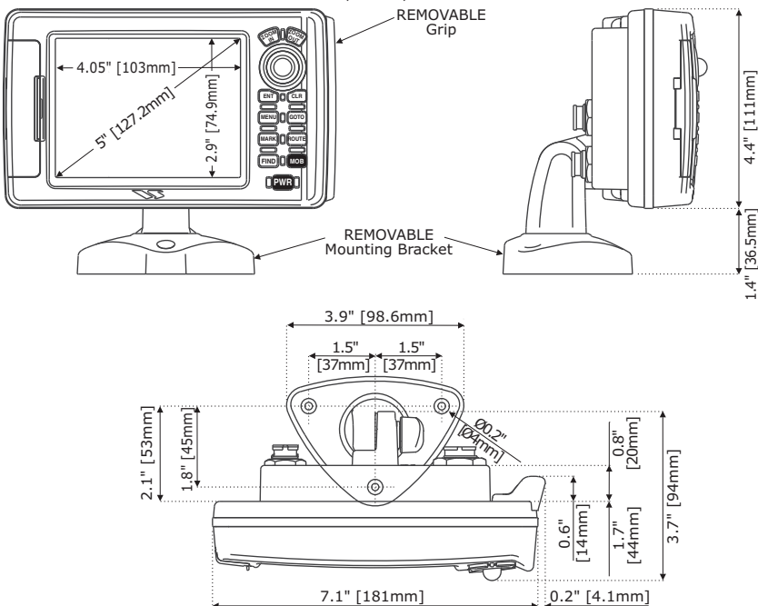
Figure 20.0 - CPF180i Dimensions [inch/mm]
