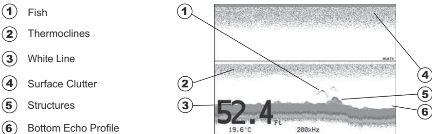
Figure 17.1.1 - The Fish Finder display
